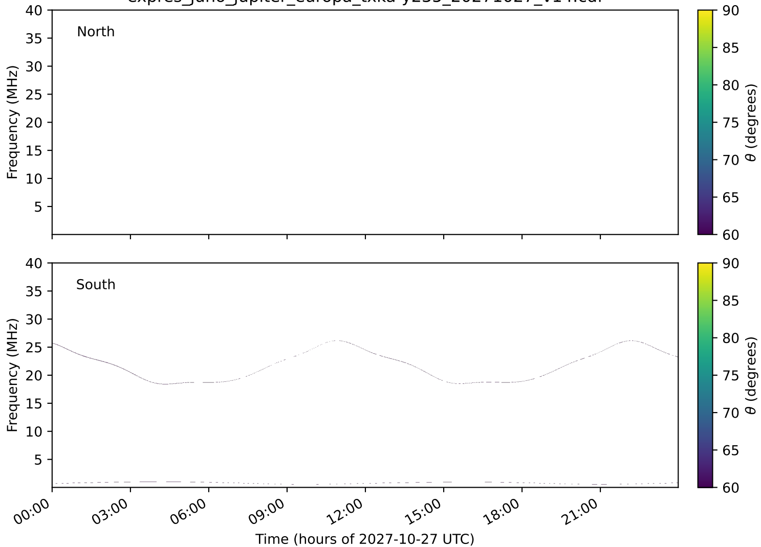
expres_juno_jupiter_europa_txka-y235_20271027_v14.cdf
