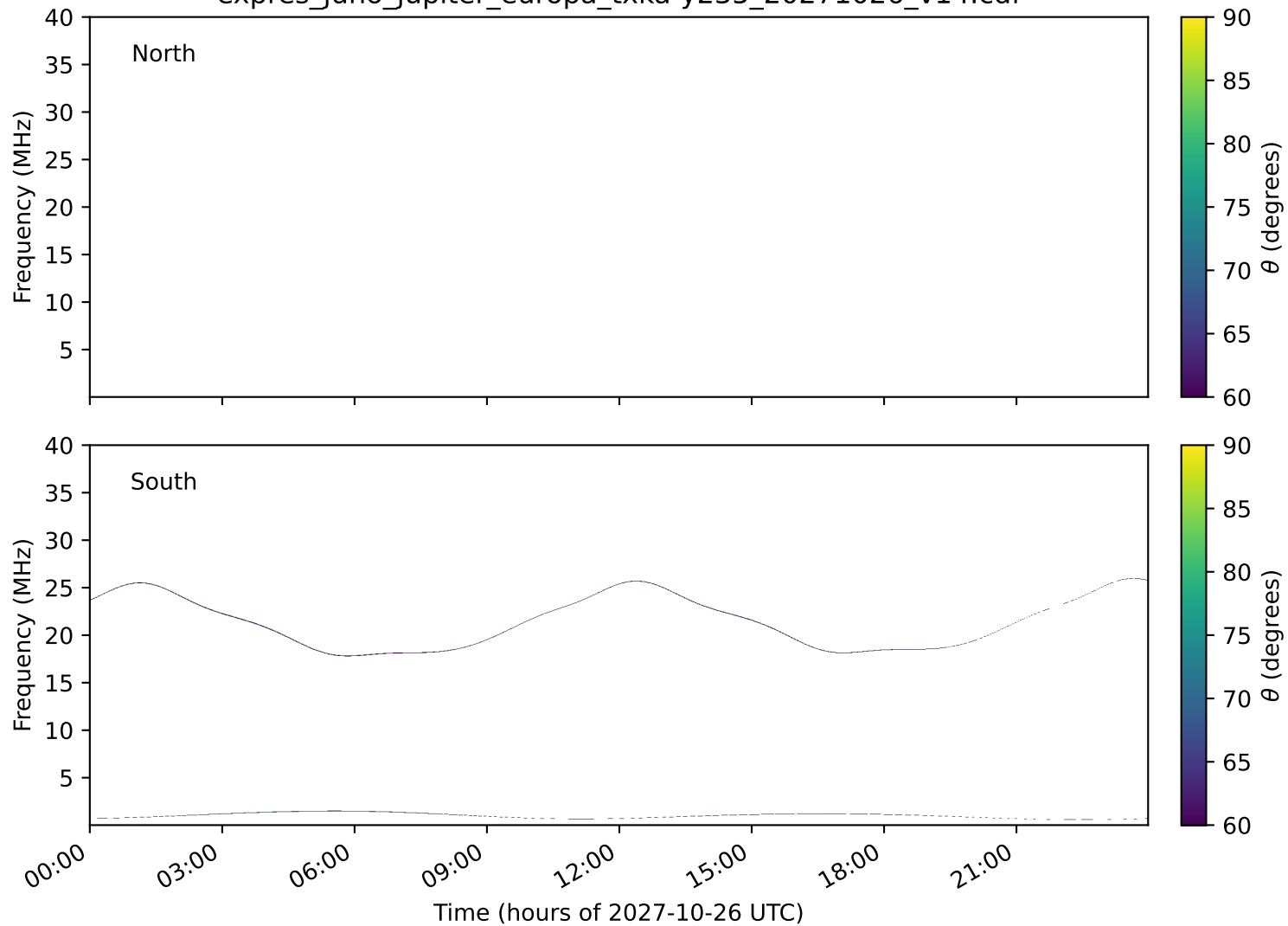
expres_juno_jupiter_europa_txka-y235_20271026_v14.cdf
