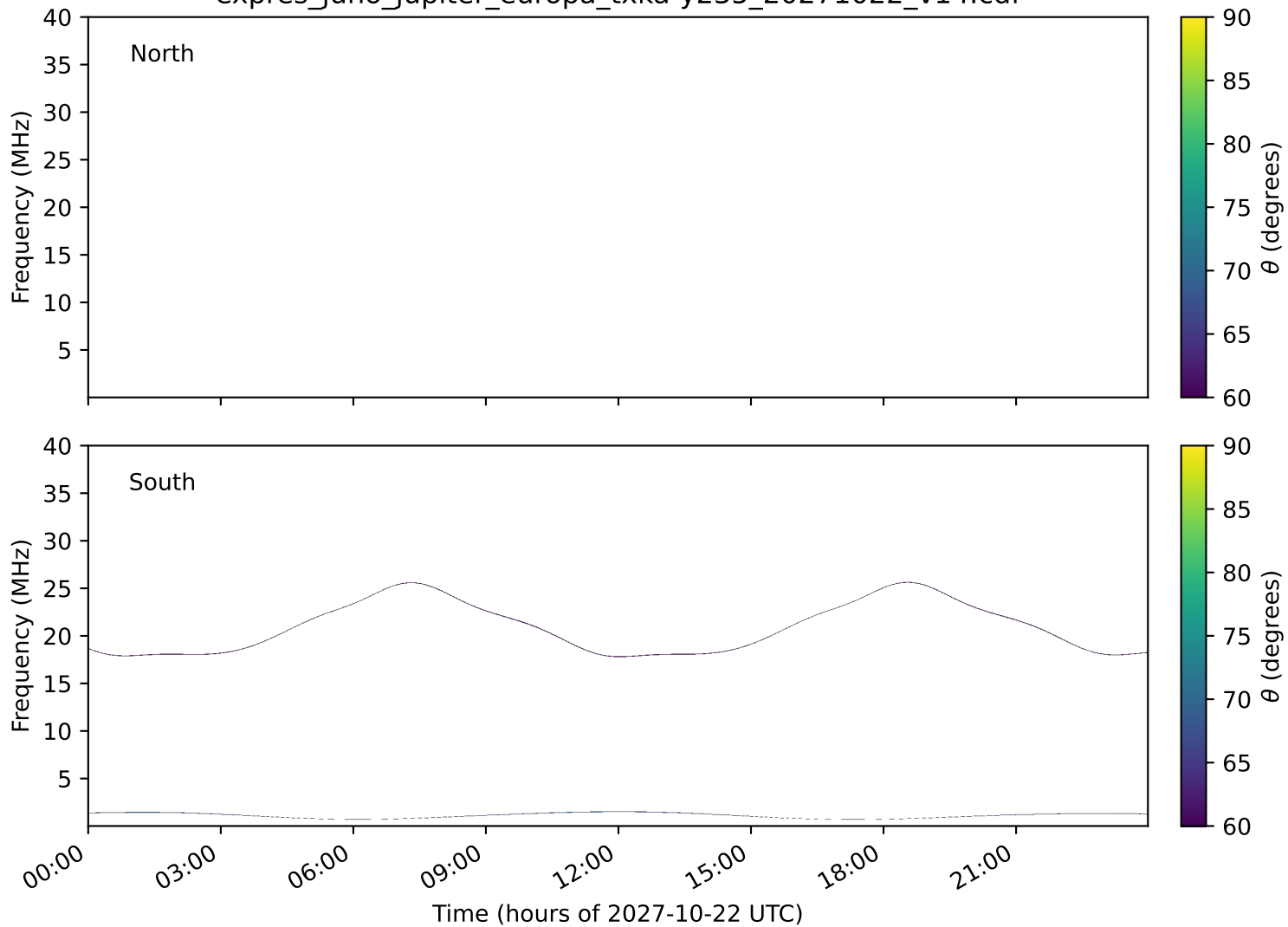
expres_juno_jupiter_europa_txka-y235_20271022_v14.cdf
