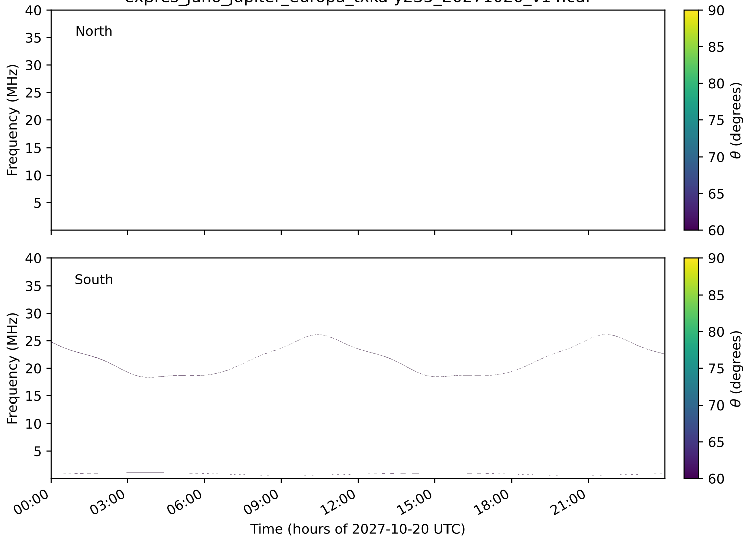
expres_juno_jupiter_europa_txka-y235_20271020_v14.cdf
