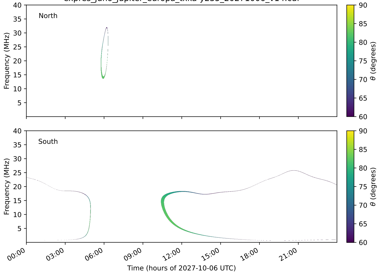
expres_juno_jupiter_europa_txka-y235_20271006_v14.cdf
