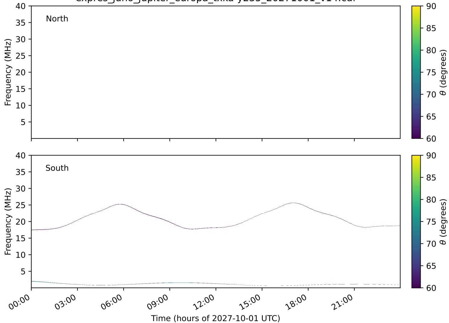
expres_juno_jupiter_europa_txka-y235_20271001_v14.cdf
