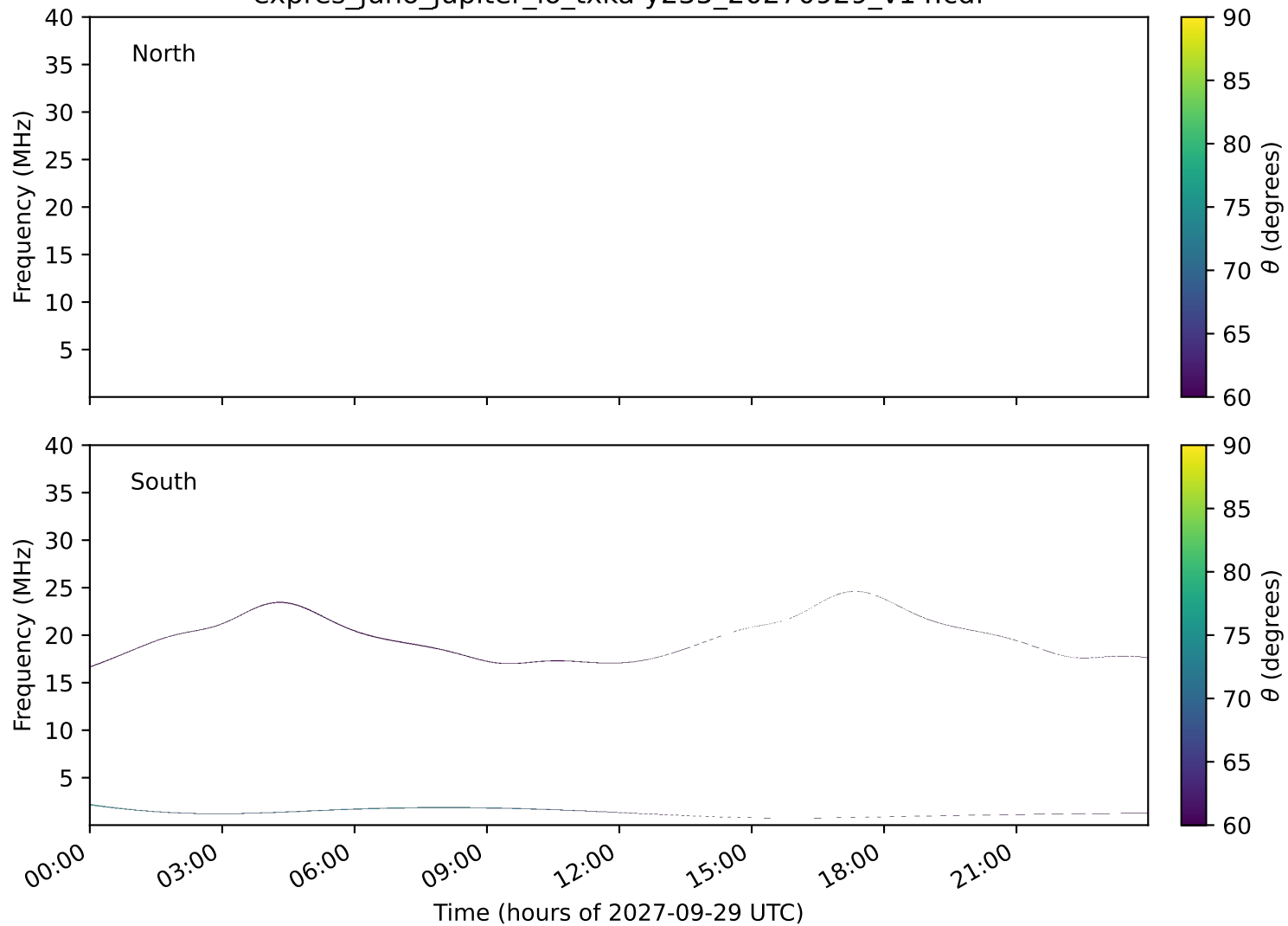
expres_juno_jupiter_io_txka-y235_20270929_v14.cdf
