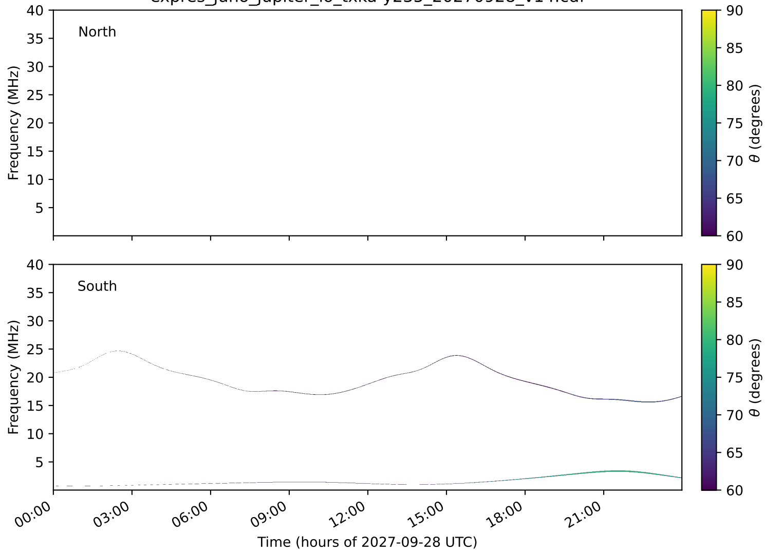
expres_juno_jupiter_io_txka-y235_20270928_v14.cdf
