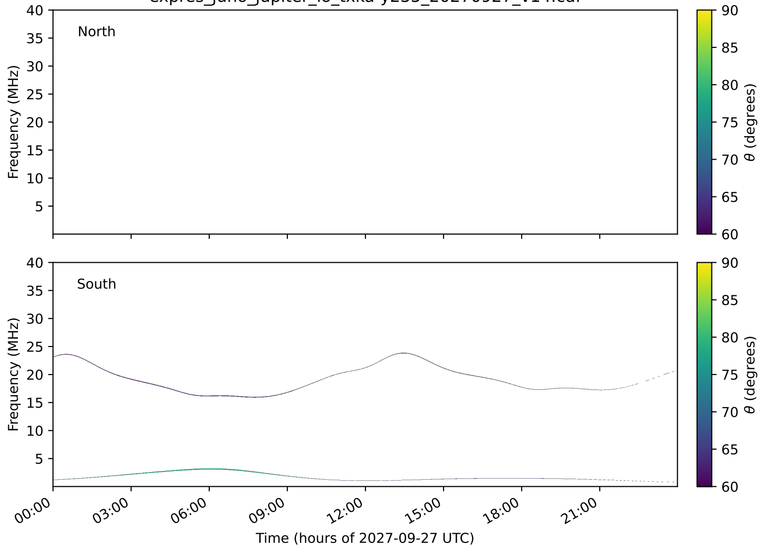
expres_juno_jupiter_io_txka-y235_20270927_v14.cdf
