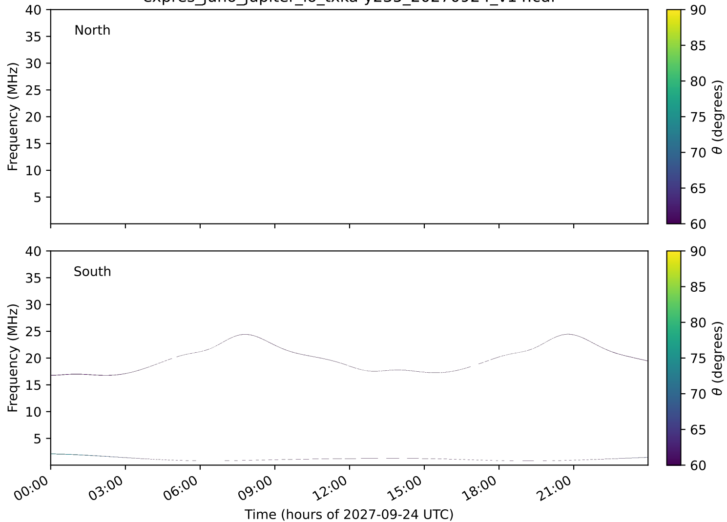
expres_juno_jupiter_io_txka-y235_20270924_v14.cdf
