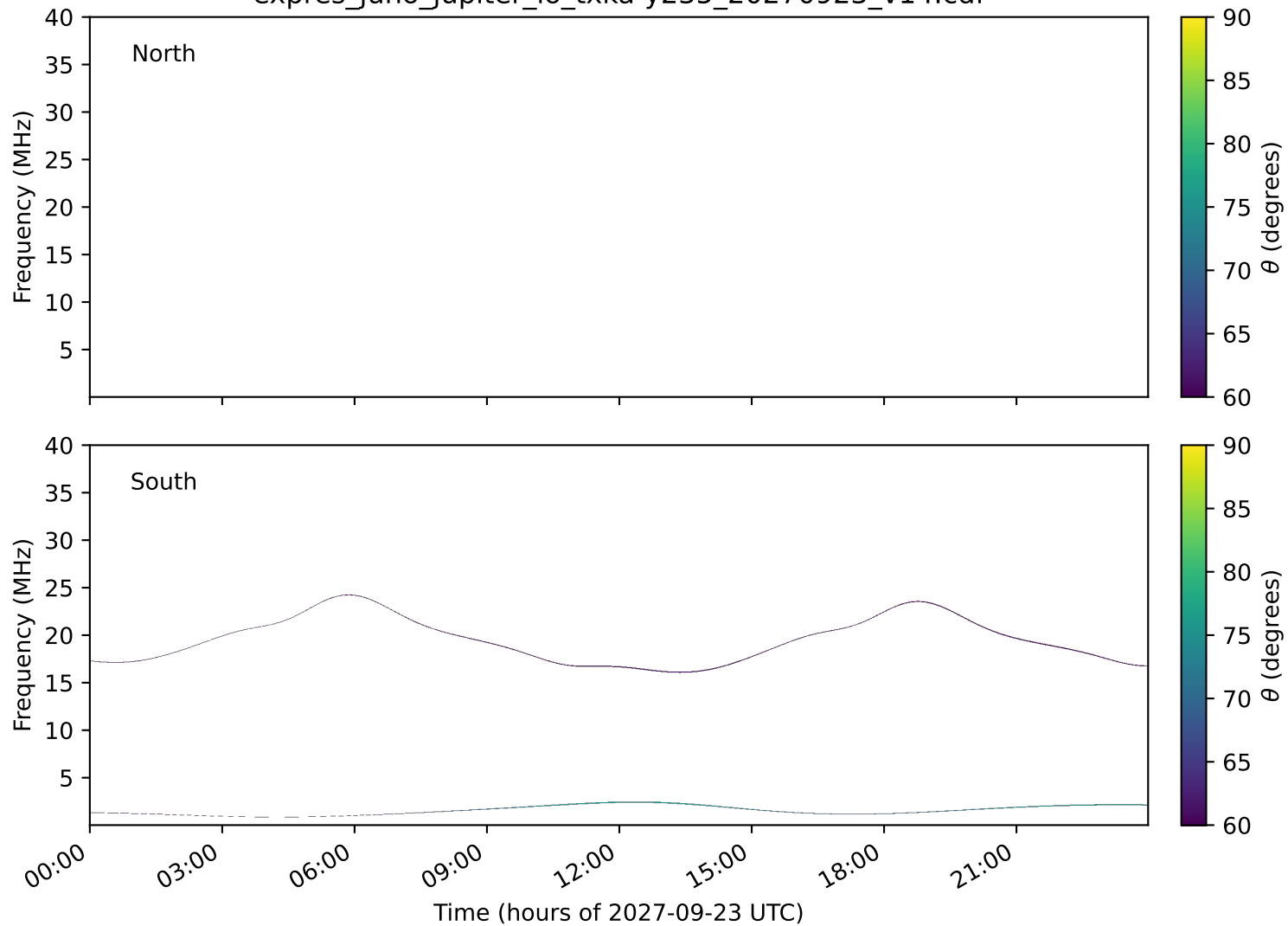
expres_juno_jupiter_io_txka-y235_20270923_v14.cdf
