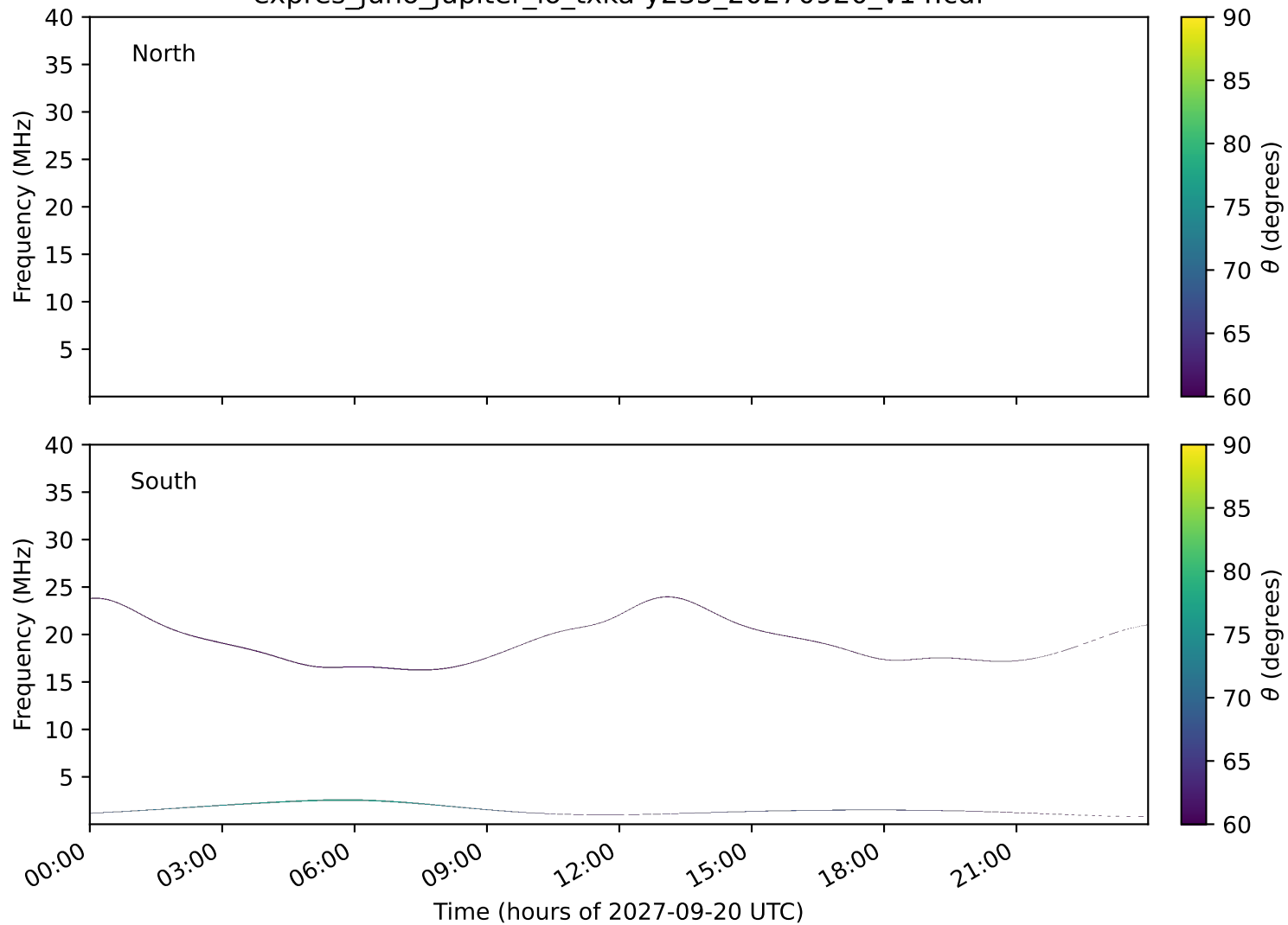
expres_juno_jupiter_io_txka-y235_20270920_v14.cdf
