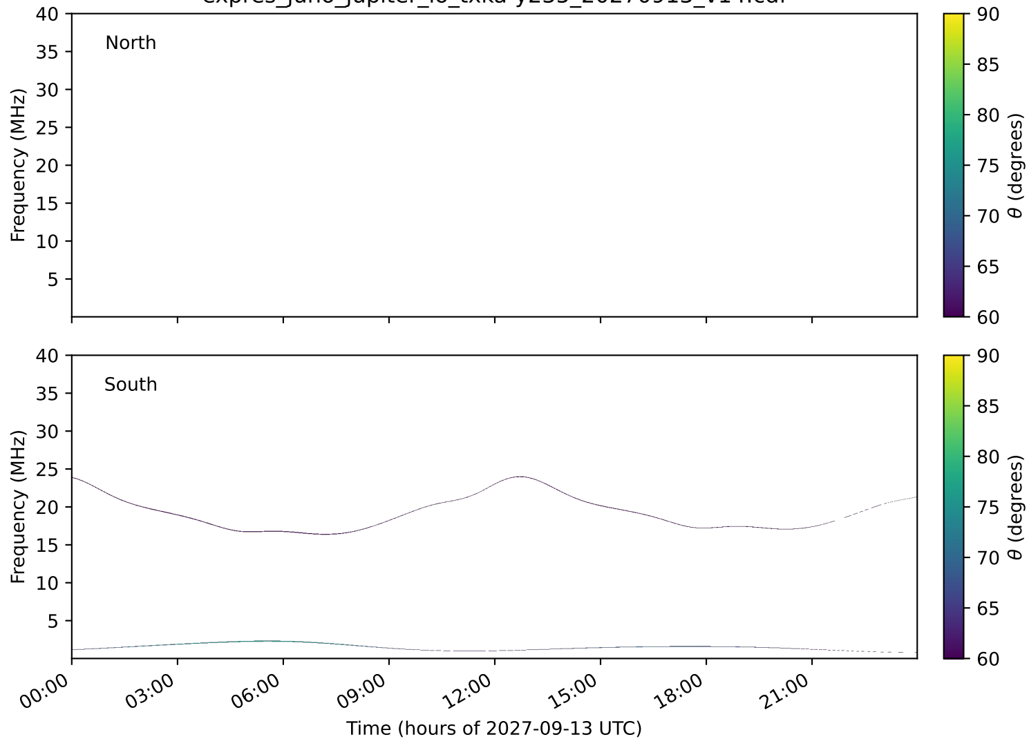
expres_juno_jupiter_io_txka-y235_20270913_v14.cdf
