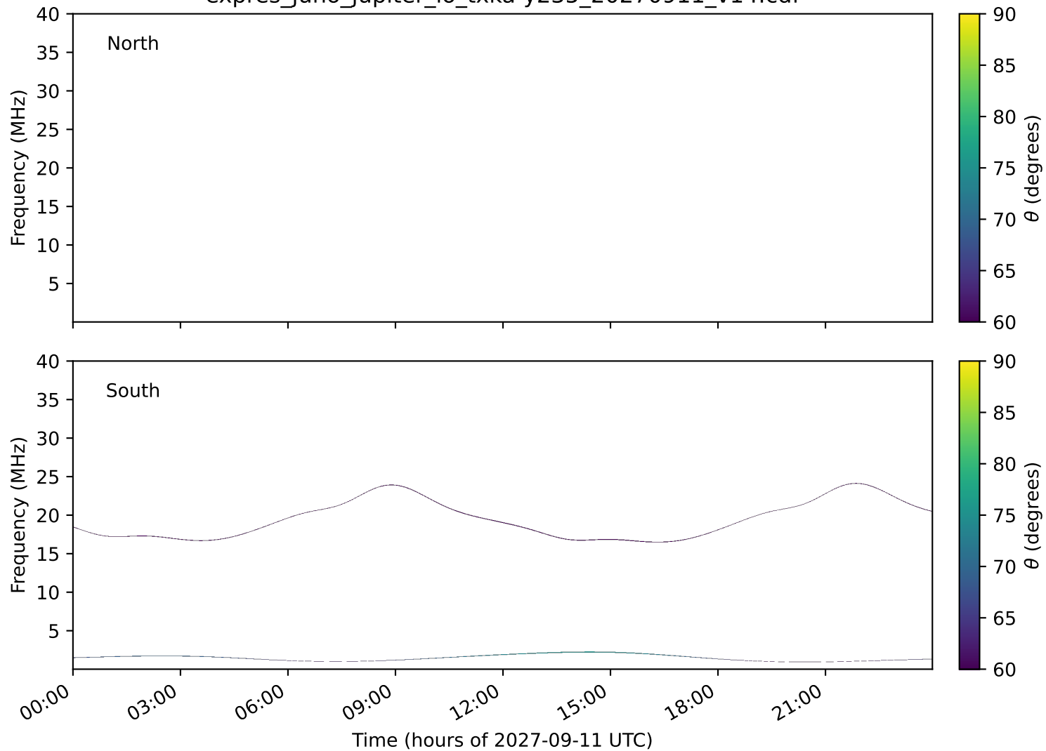
expres_juno_jupiter_io_txka-y235_20270911_v14.cdf
