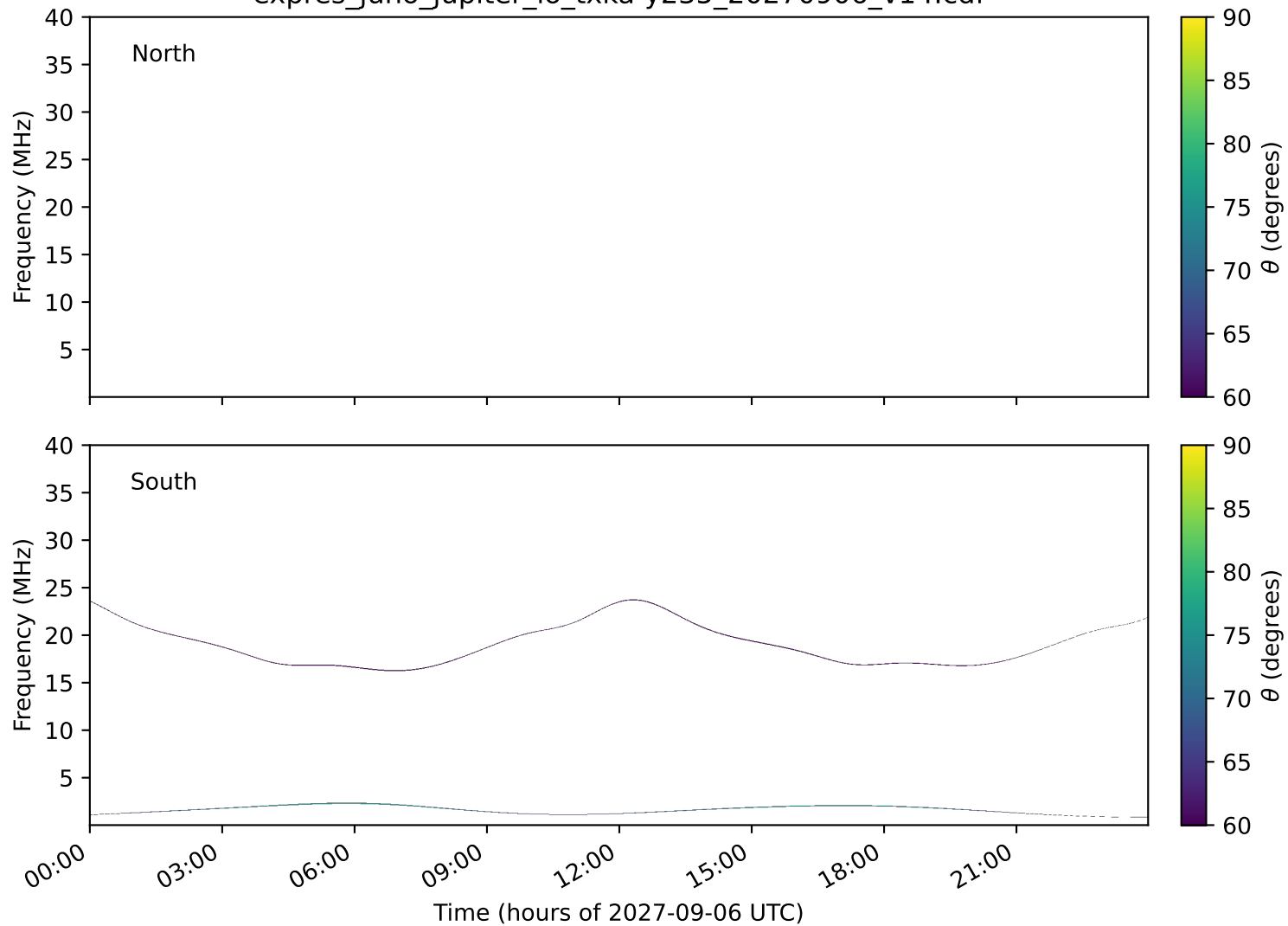
expres_juno_jupiter_io_txka-y235_20270906_v14.cdf
