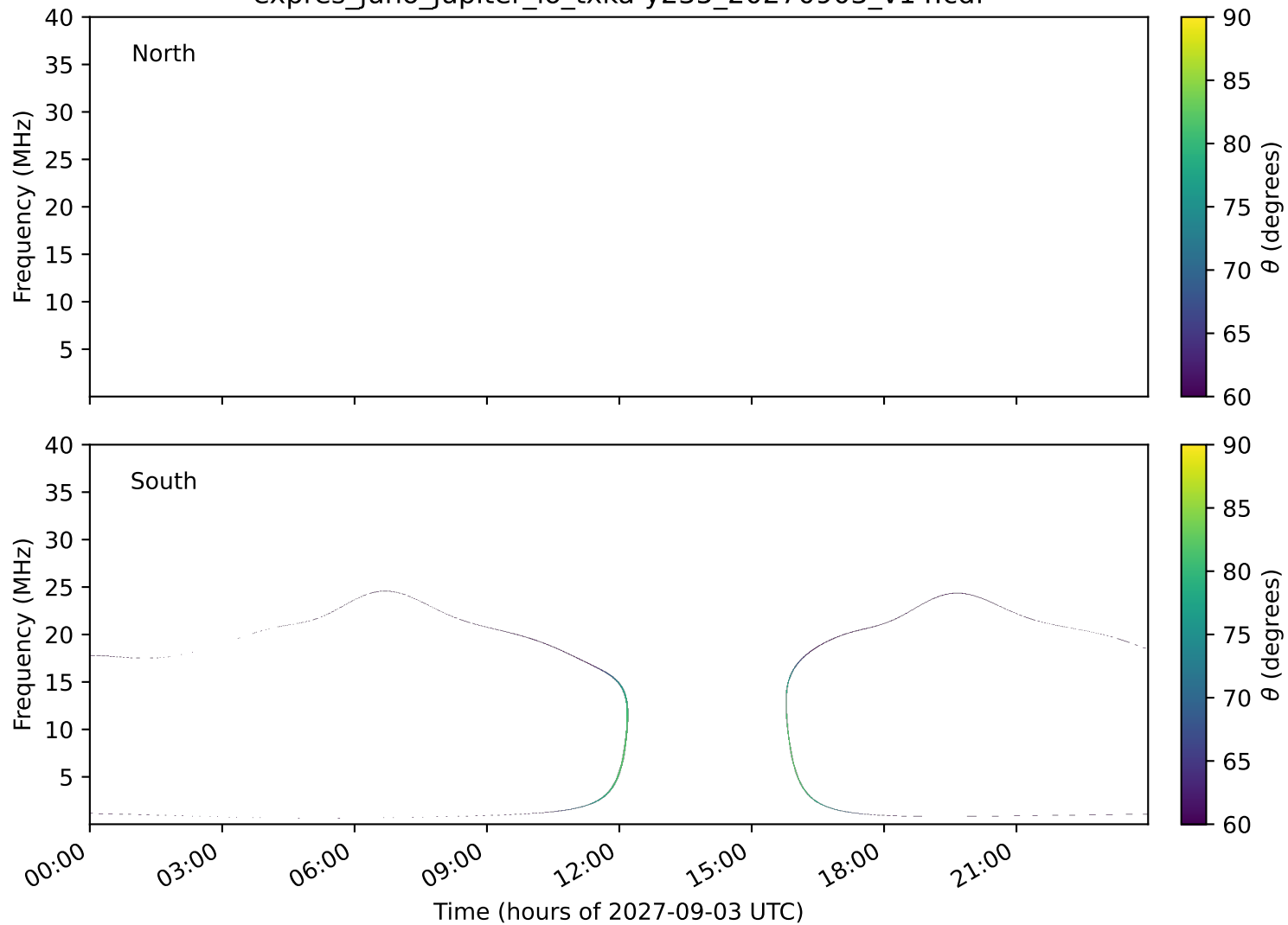
expres_juno_jupiter_io_txka-y235_20270903_v14.cdf
