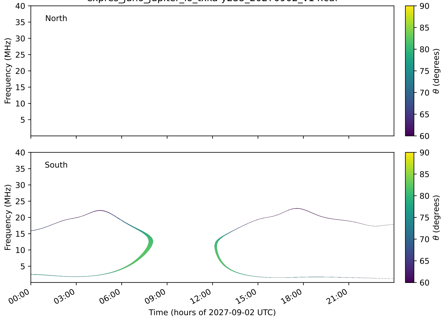
expres_juno_jupiter_io_txka-y235_20270902_v14.cdf
