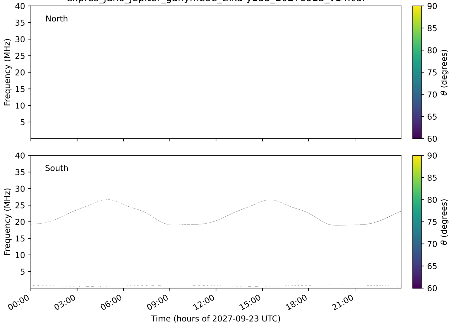
expres_juno_jupiter_ganymede_txka-y235_20270923_v14.cdf
