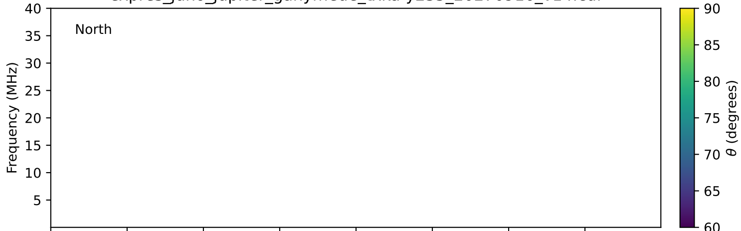
expres_juno_jupiter_ganymede_txka-y235_20270916_v14.cdf
