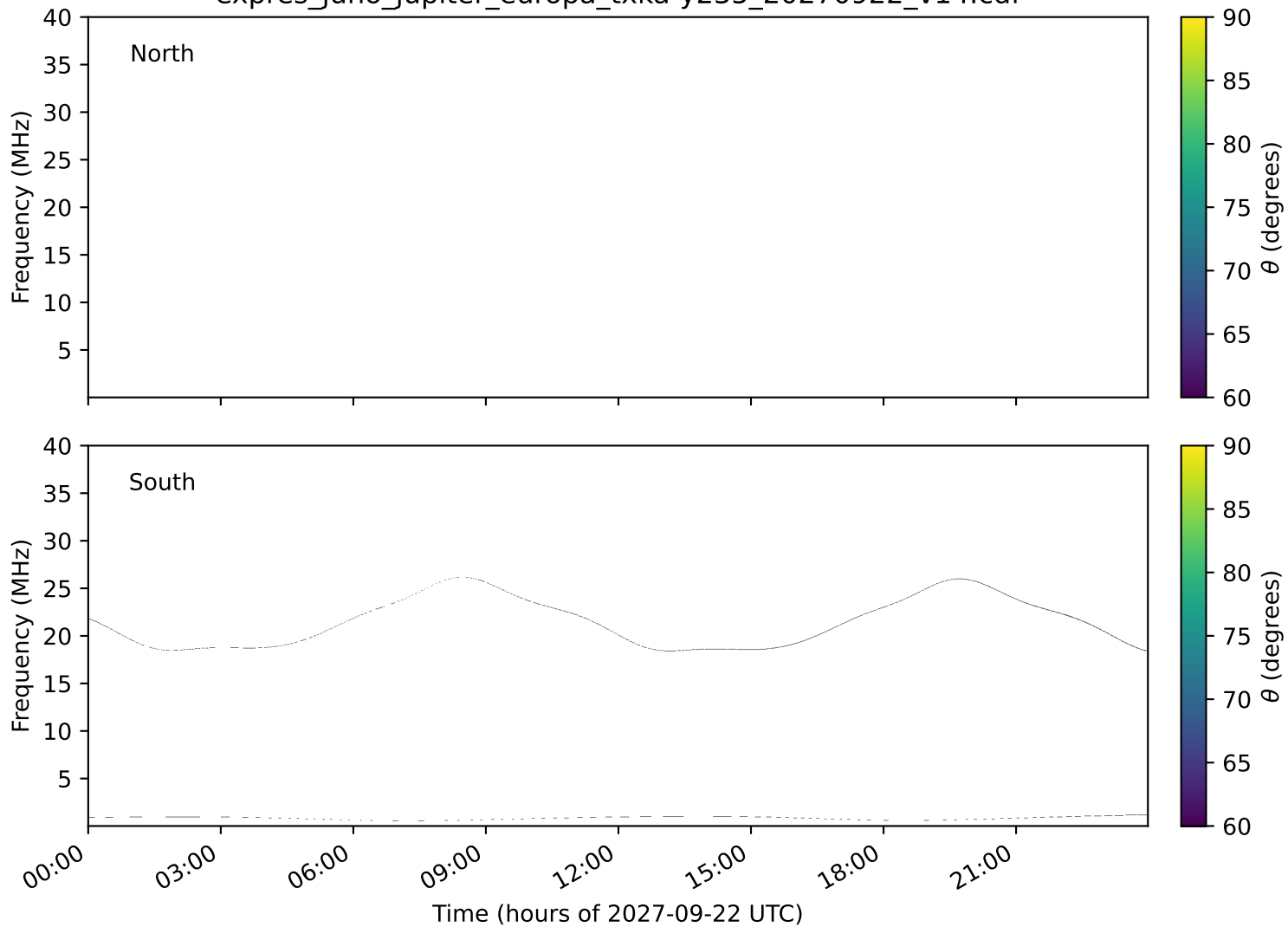
expres_juno_jupiter_europa_txka-y235_20270922_v14.cdf
