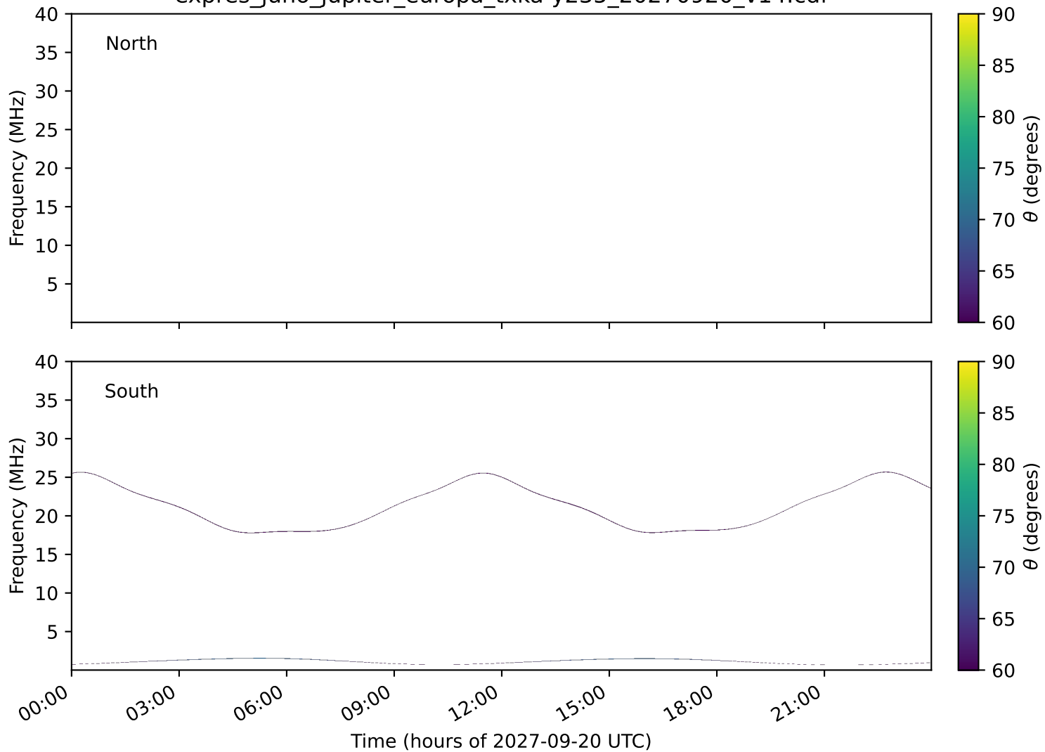
expres_juno_jupiter_europa_txka-y235_20270920_v14.cdf
