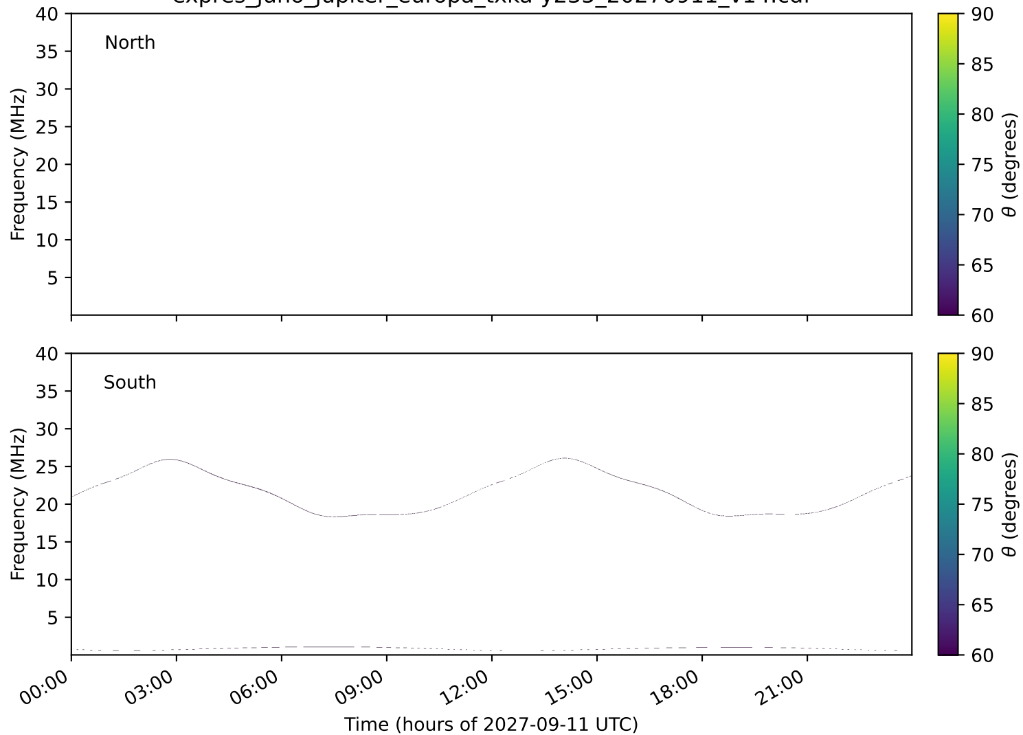
expres_juno_jupiter_europa_txka-y235_20270911_v14.cdf
