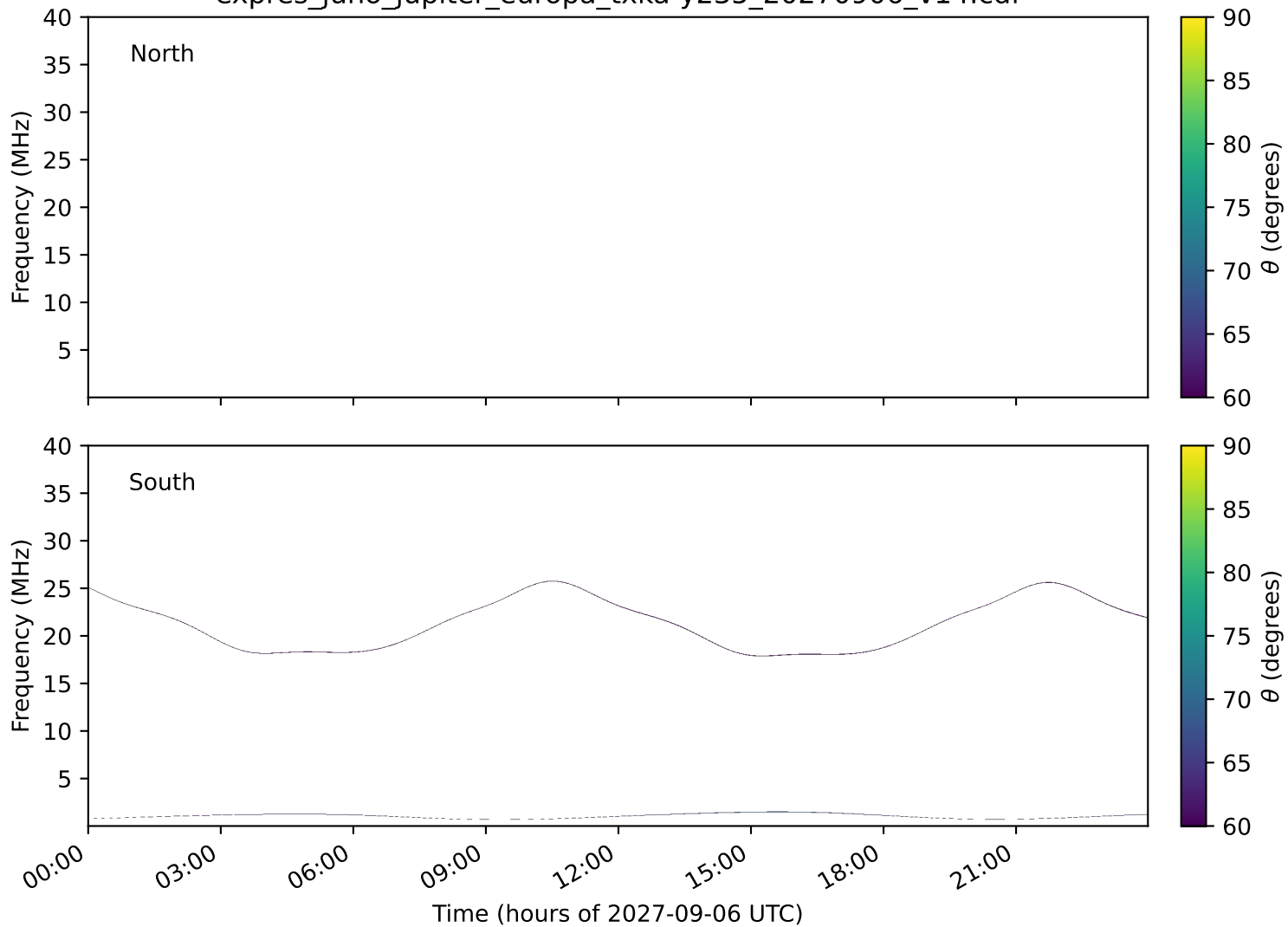
expres_juno_jupiter_europa_txka-y235_20270906_v14.cdf
