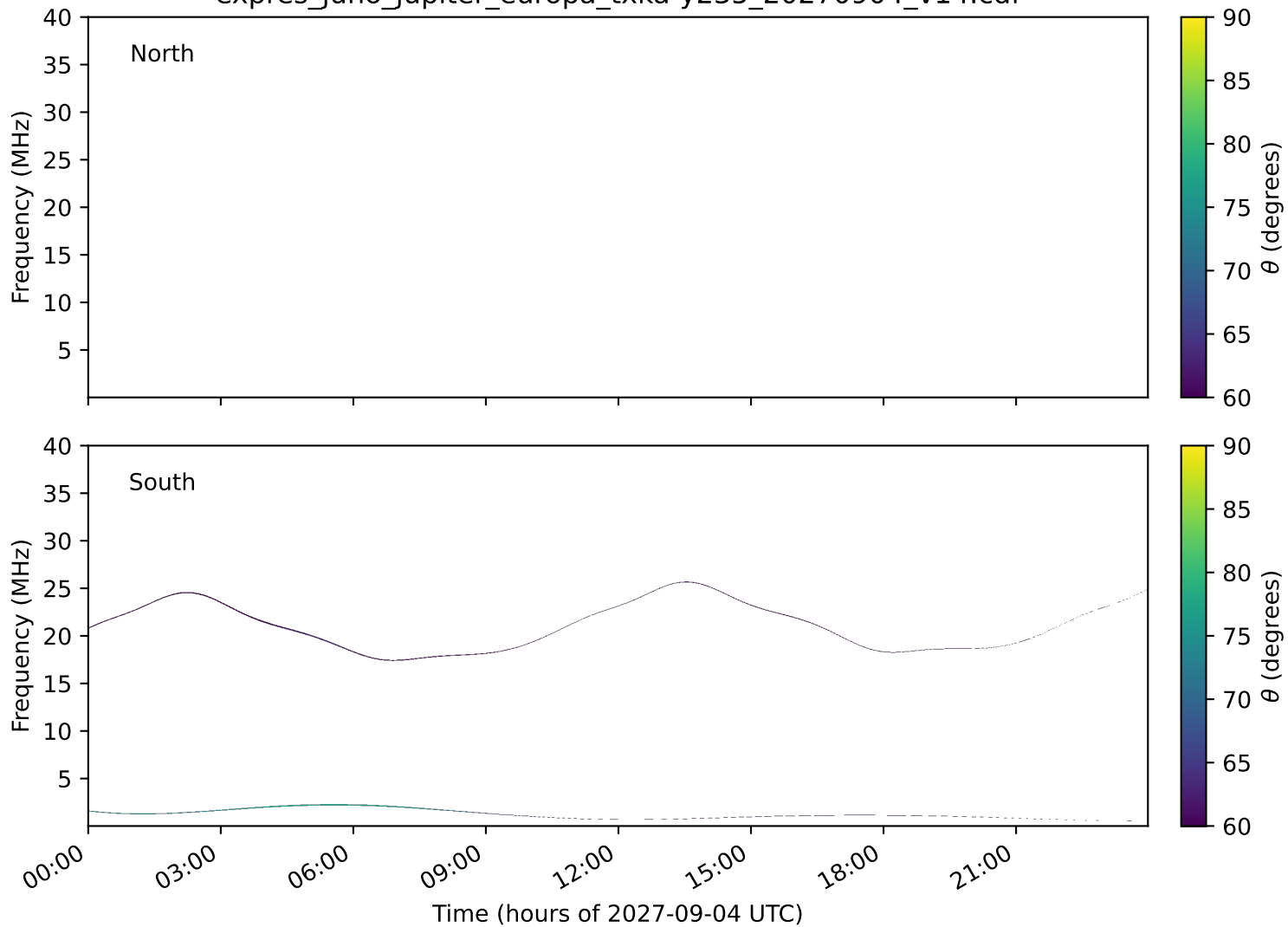
expres_juno_jupiter_europa_txka-y235_20270904_v14.cdf
