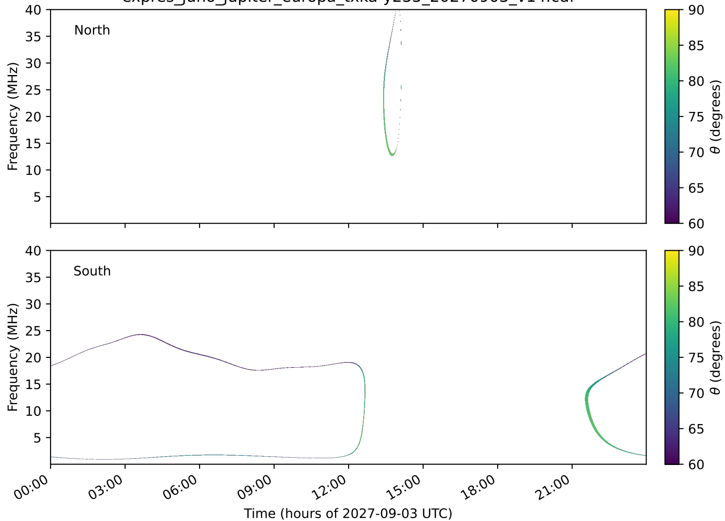
expres_juno_jupiter_europa_txka-y235_20270903_v14.cdf
