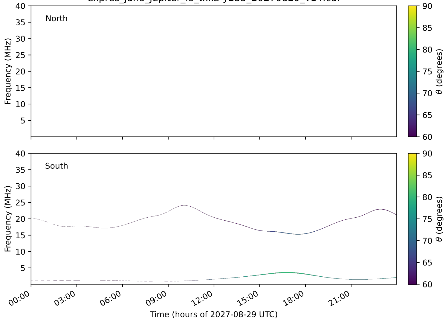
expres_juno_jupiter_io_txka-y235_20270829_v14.cdf
