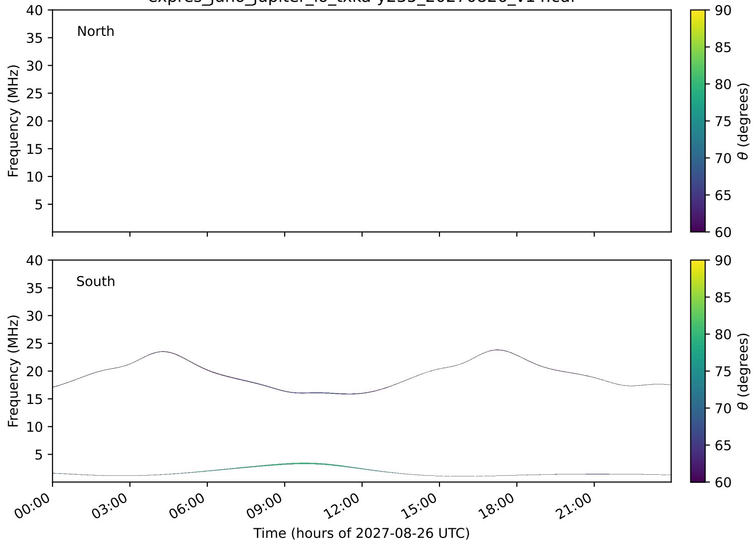
expres_juno_jupiter_io_txka-y235_20270826_v14.cdf
