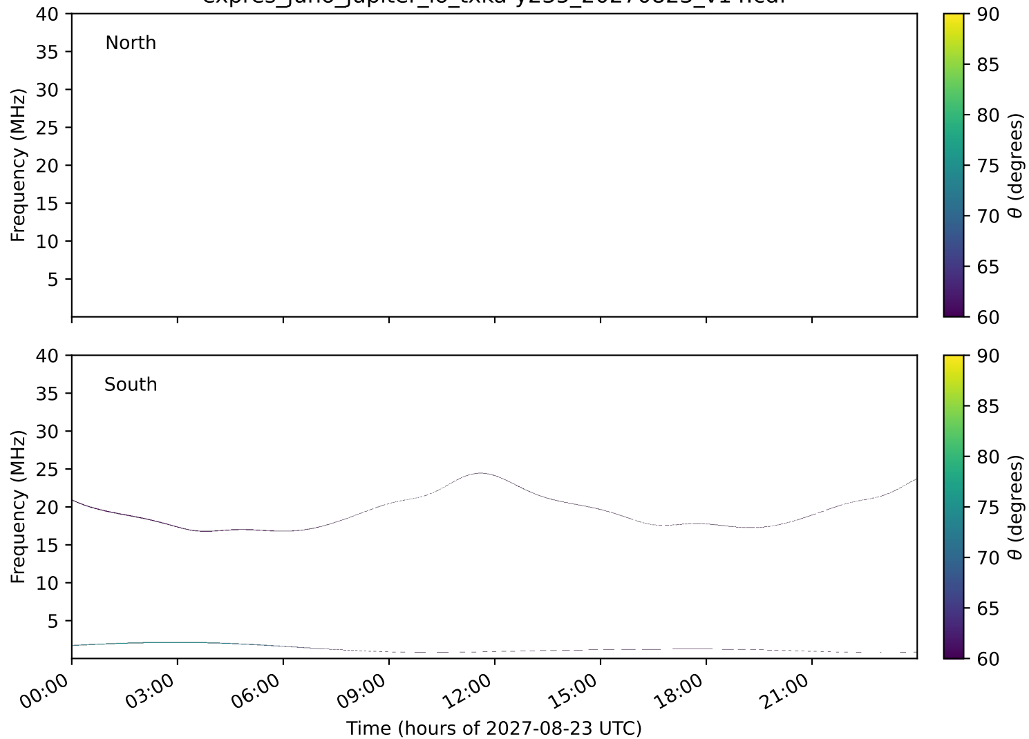
expres_juno_jupiter_io_txka-y235_20270823_v14.cdf
