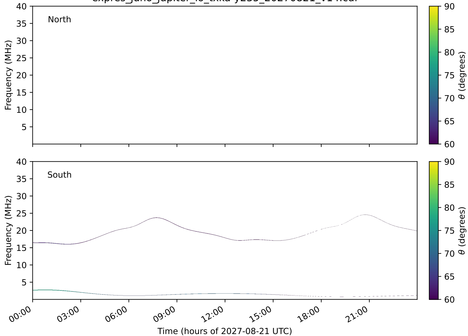
expres_juno_jupiter_io_txka-y235_20270821_v14.cdf
