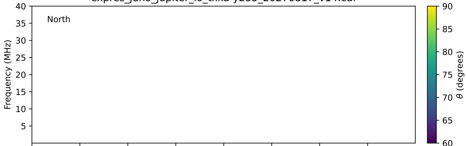
expres_juno_jupiter_io_txka-y235_20270817_v14.cdf
