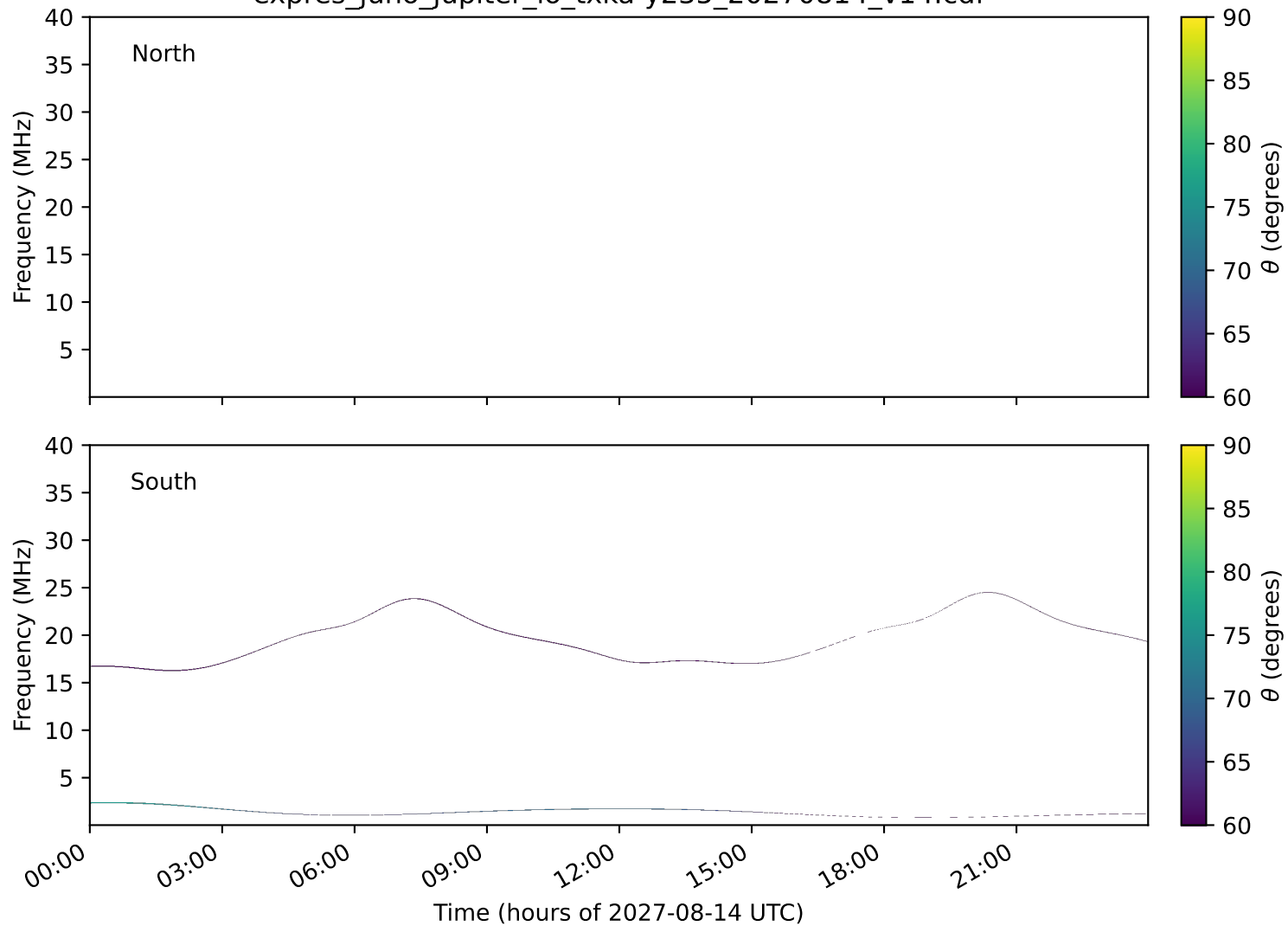
expres_juno_jupiter_io_txka-y235_20270814_v14.cdf
