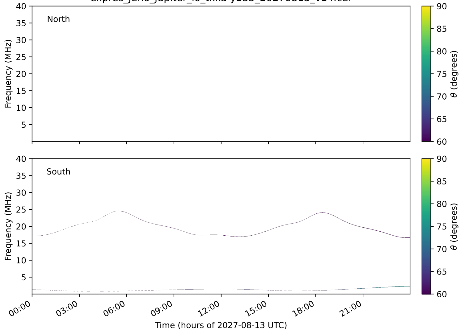
expres_juno_jupiter_io_txka-y235_20270813_v14.cdf
