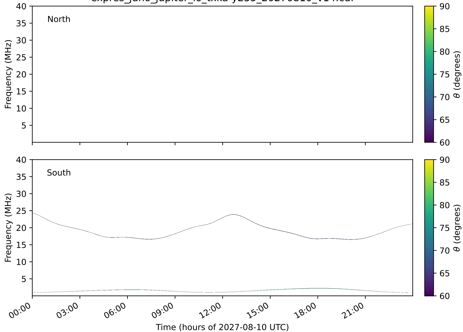
expres_juno_jupiter_io_txka-y235_20270810_v14.cdf
