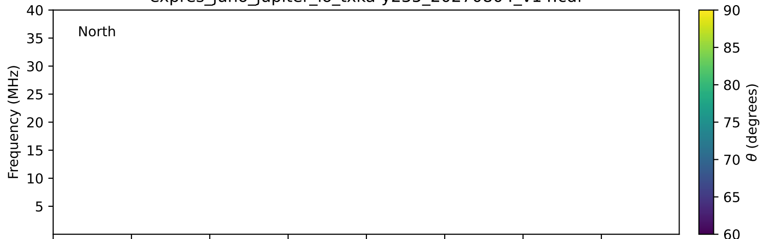
expres_juno_jupiter_io_txka-y235_20270804_v14.cdf
