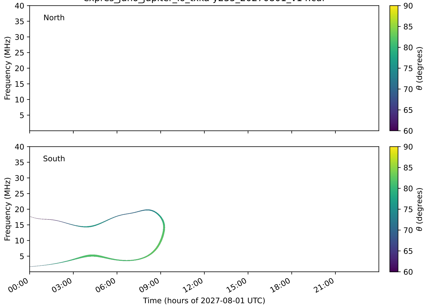
expres_juno_jupiter_io_txka-y235_20270801_v14.cdf
