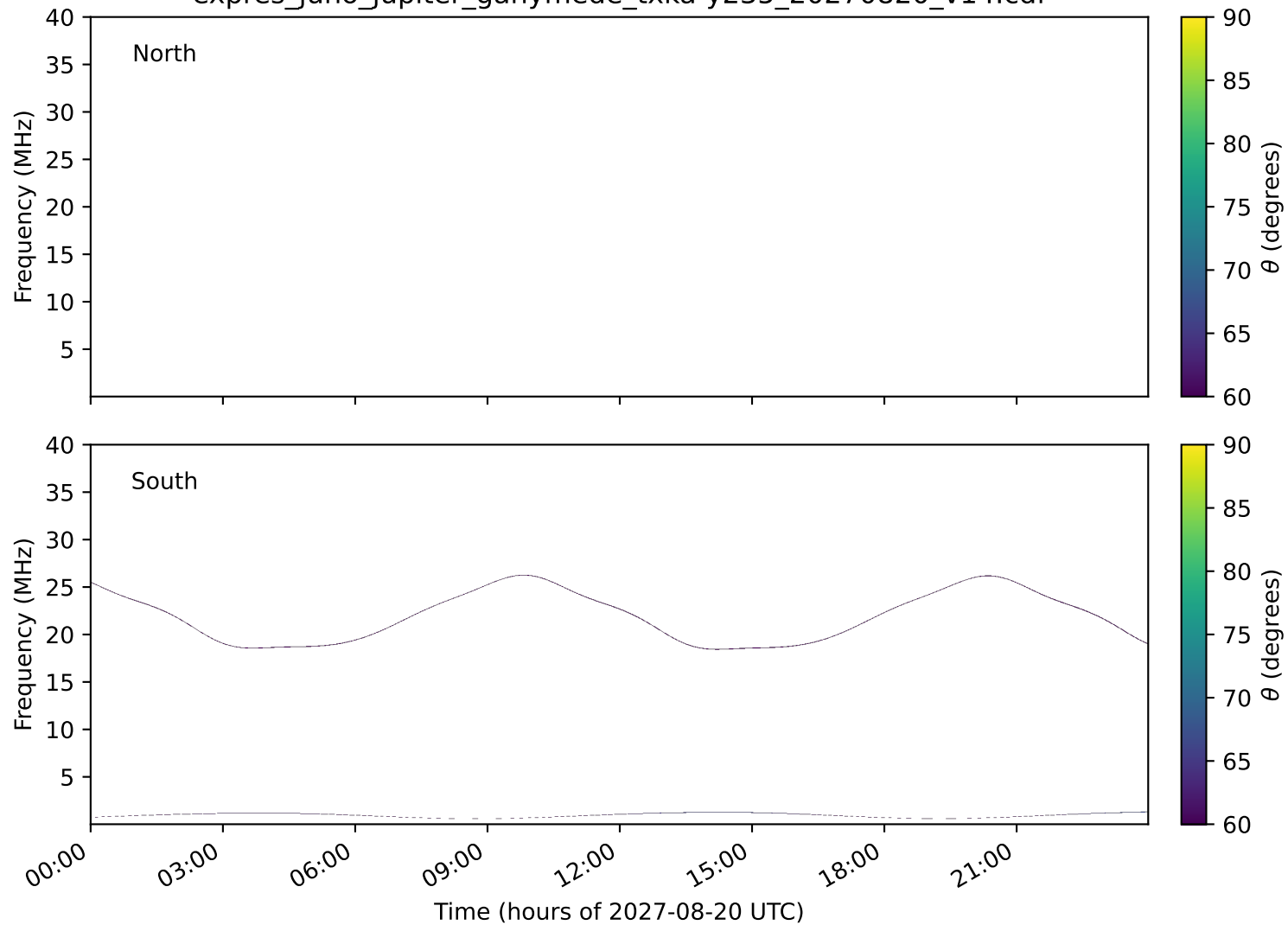
expres_juno_jupiter_ganymede_txka-y235_20270820_v14.cdf
