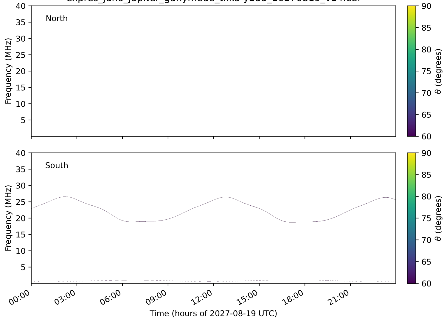
expres_juno_jupiter_ganymede_txka-y235_20270819_v14.cdf
