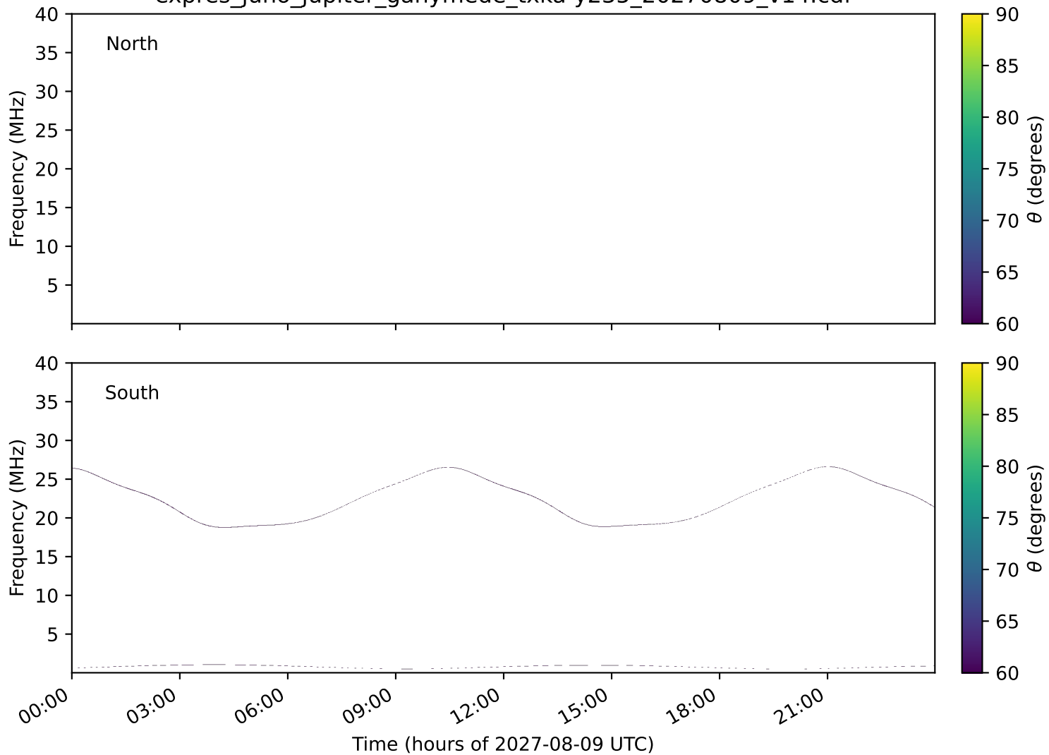
expres_juno_jupiter_ganymede_txka-y235_20270809_v14.cdf
