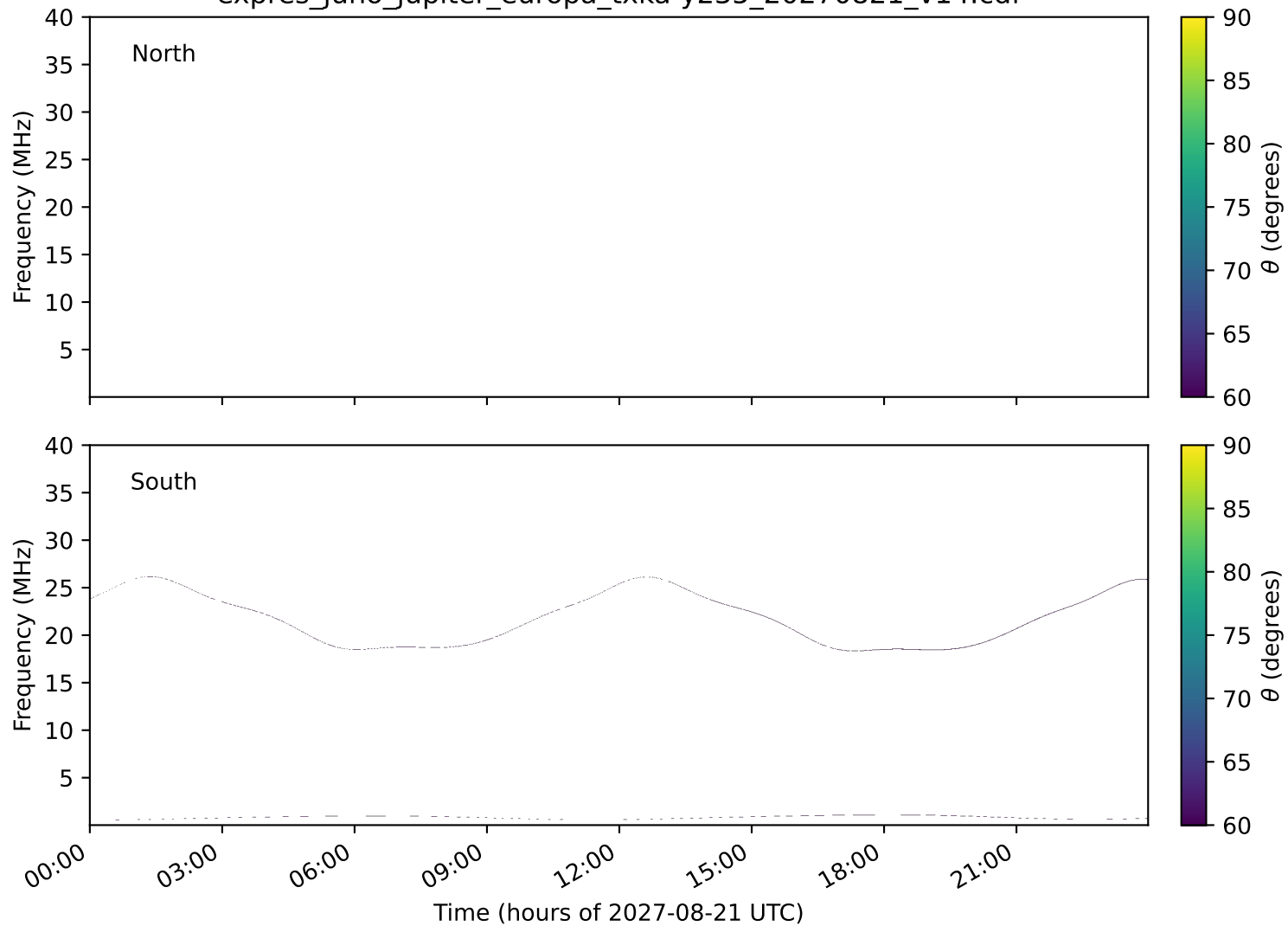
expres_juno_jupiter_europa_txka-y235_20270821_v14.cdf
