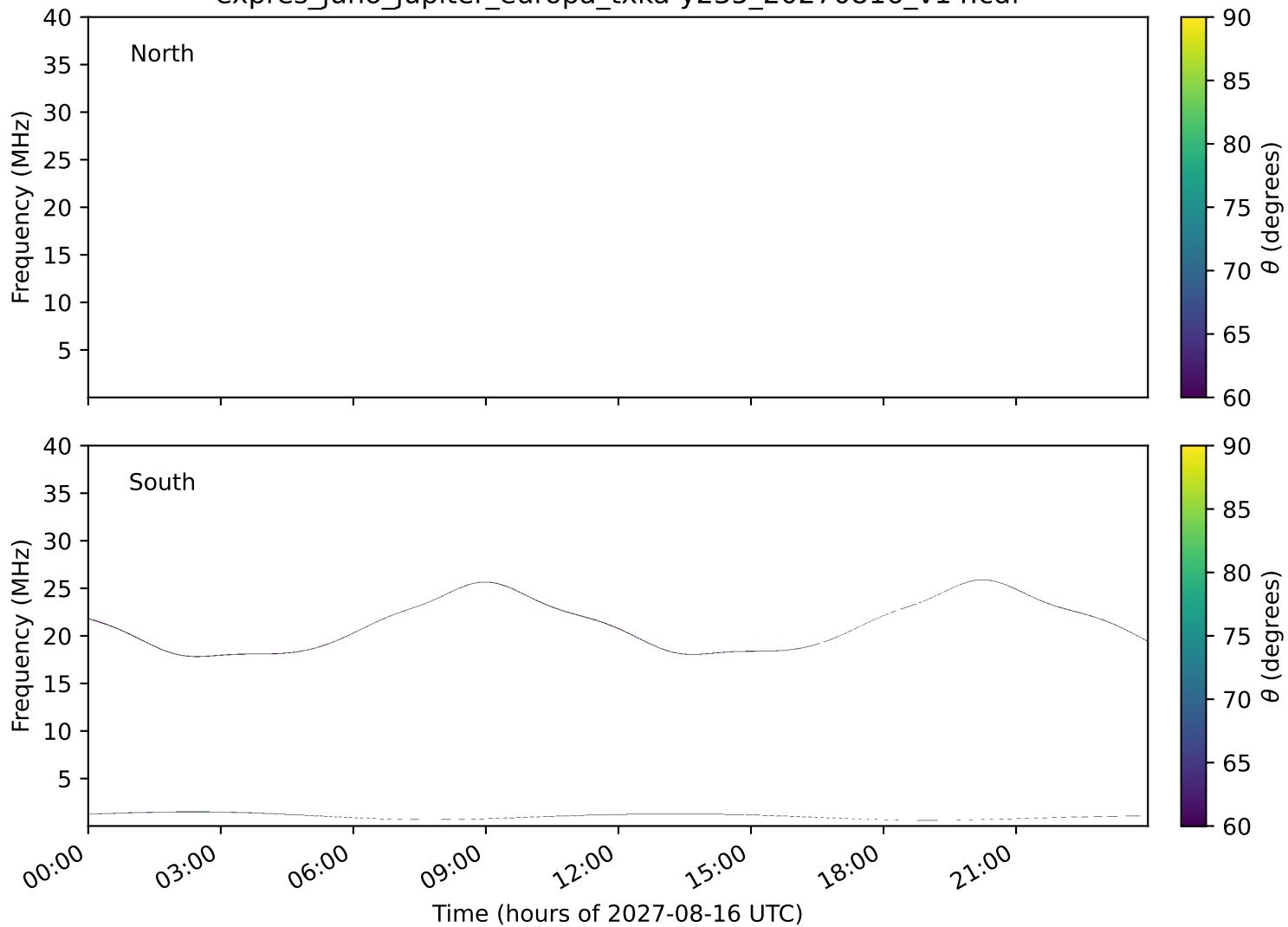
expres_juno_jupiter_europa_txka-y235_20270816_v14.cdf
