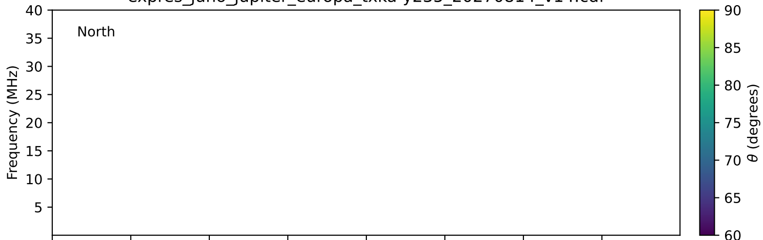
expres_juno_jupiter_europa_txka-y235_20270814_v14.cdf
