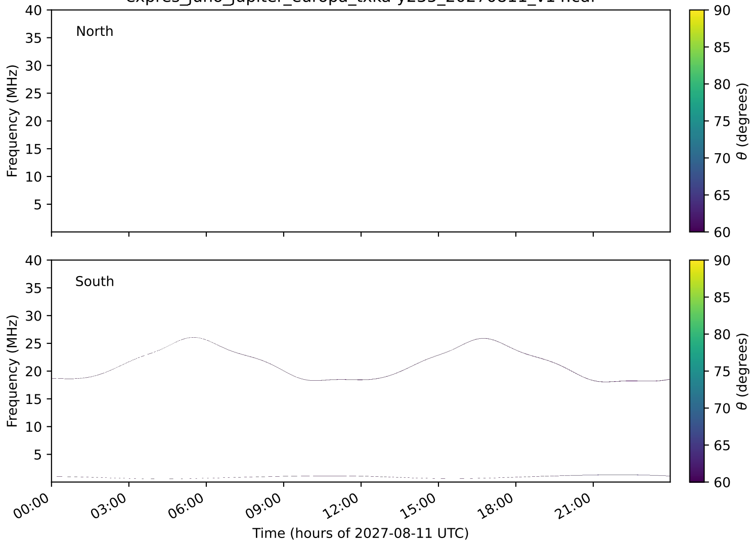
expres_juno_jupiter_europa_txka-y235_20270811_v14.cdf
