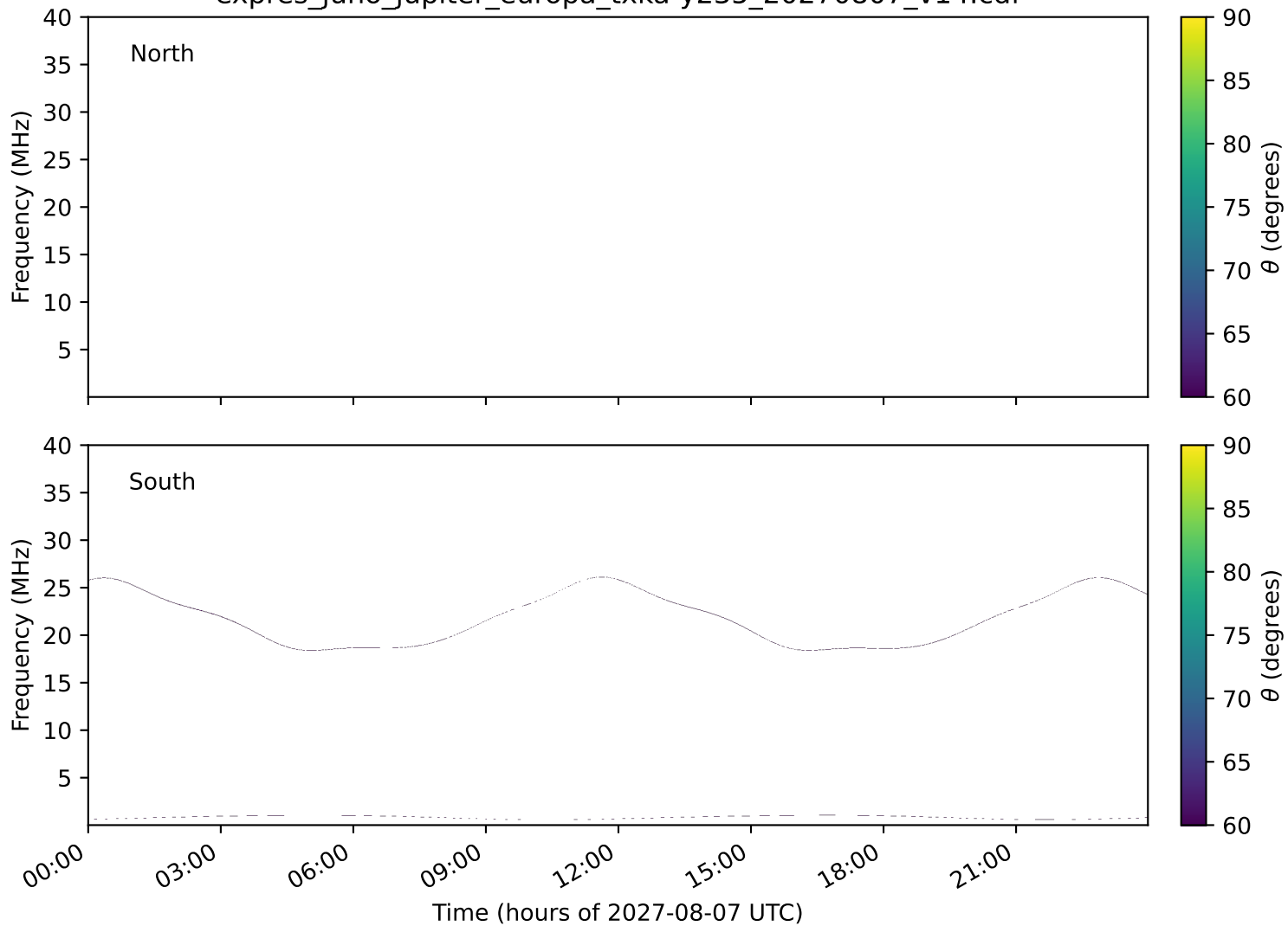
expres_juno_jupiter_europa_txka-y235_20270807_v14.cdf
