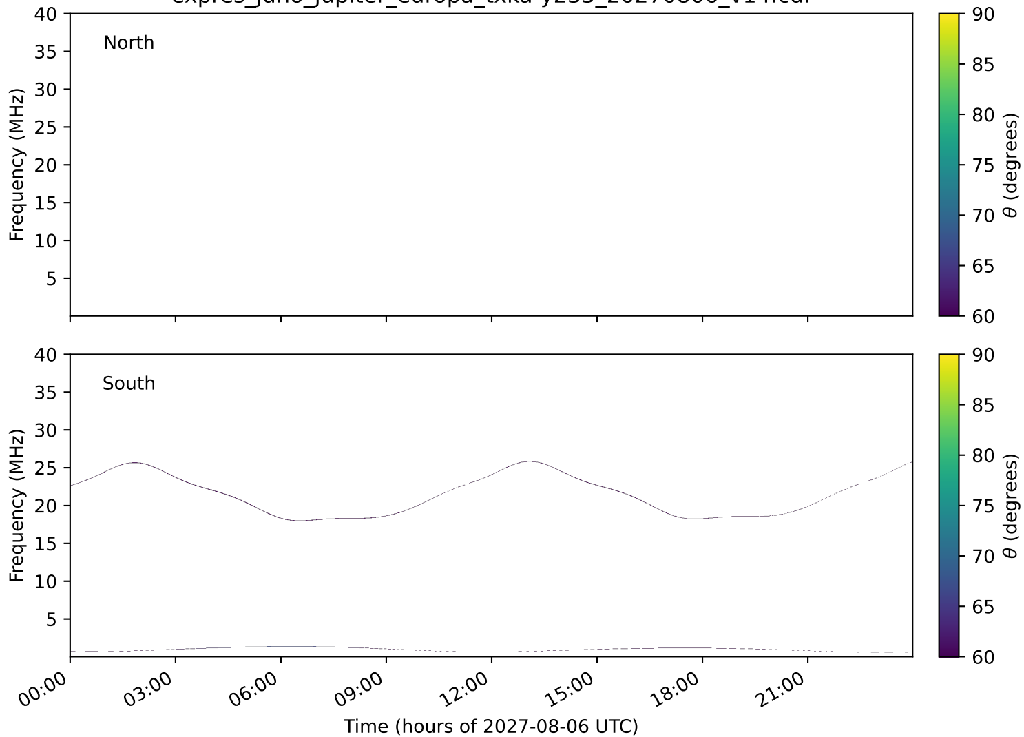
expres_juno_jupiter_europa_txka-y235_20270806_v14.cdf
