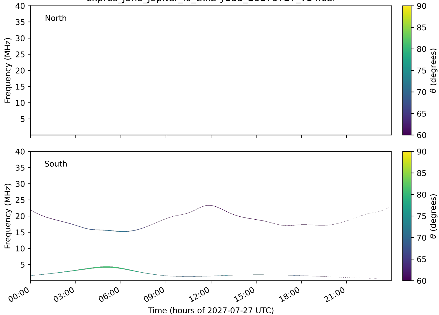
expres_juno_jupiter_io_txka-y235_20270727_v14.cdf
