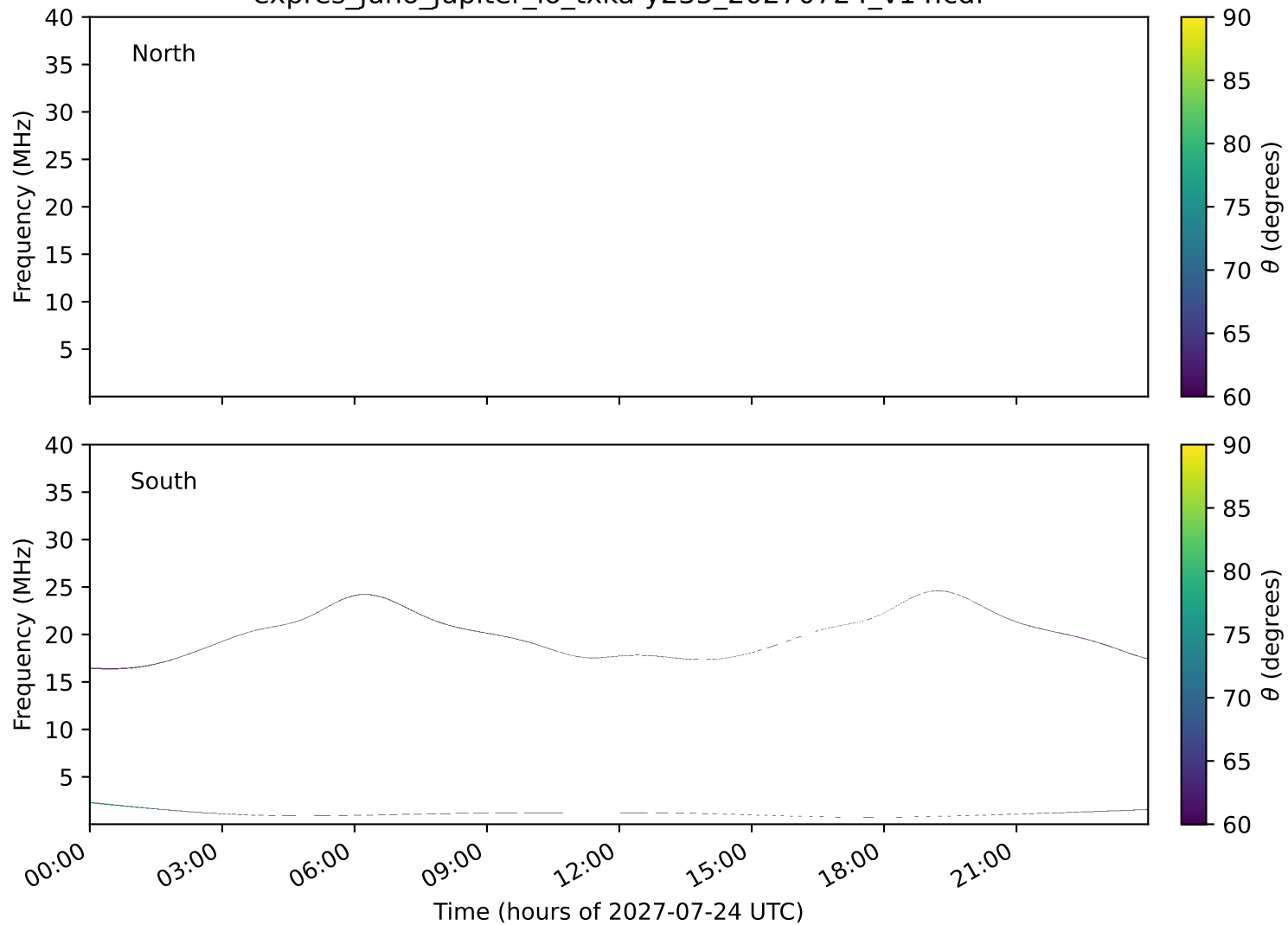
expres_juno_jupiter_io_txka-y235_20270724_v14.cdf
