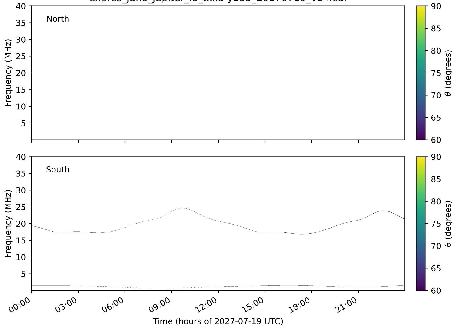
expres_juno_jupiter_io_txka-y235_20270719_v14.cdf
