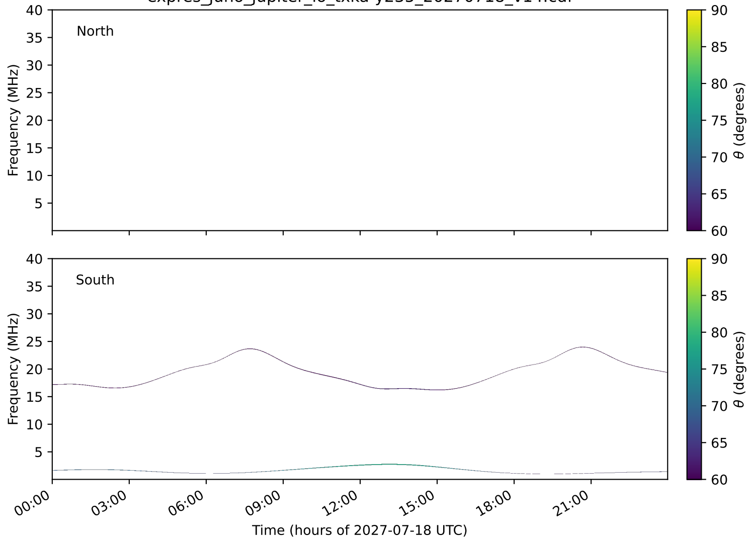
expres_juno_jupiter_io_txka-y235_20270718_v14.cdf
