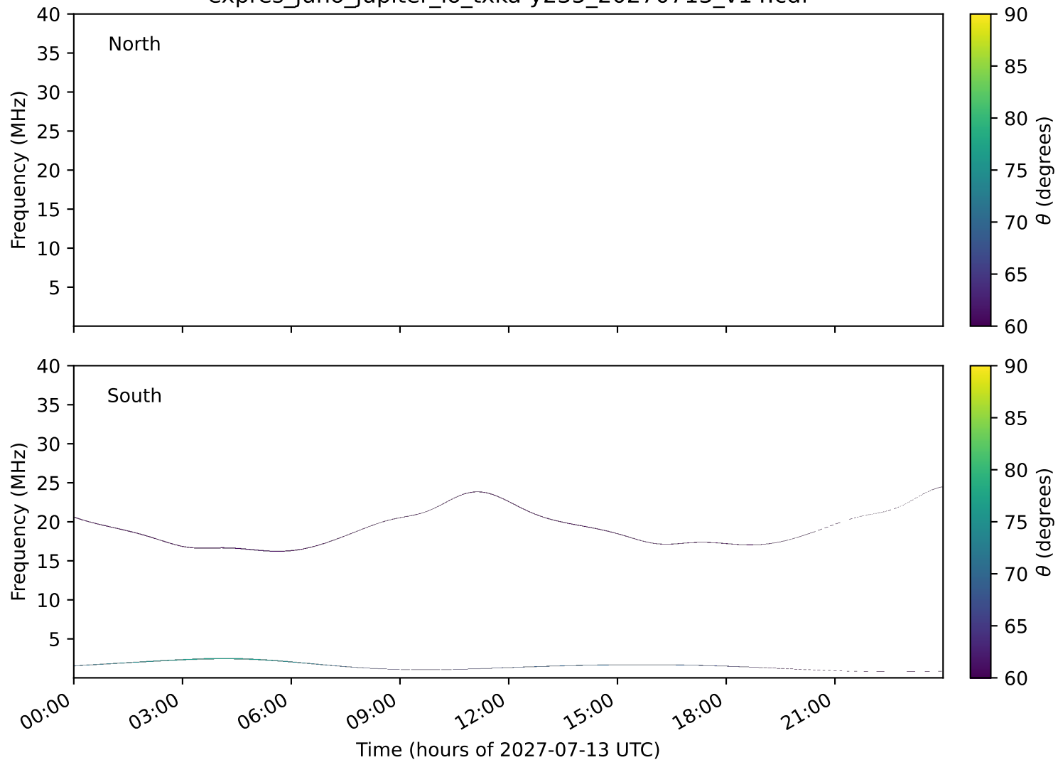
expres_juno_jupiter_io_txka-y235_20270713_v14.cdf
