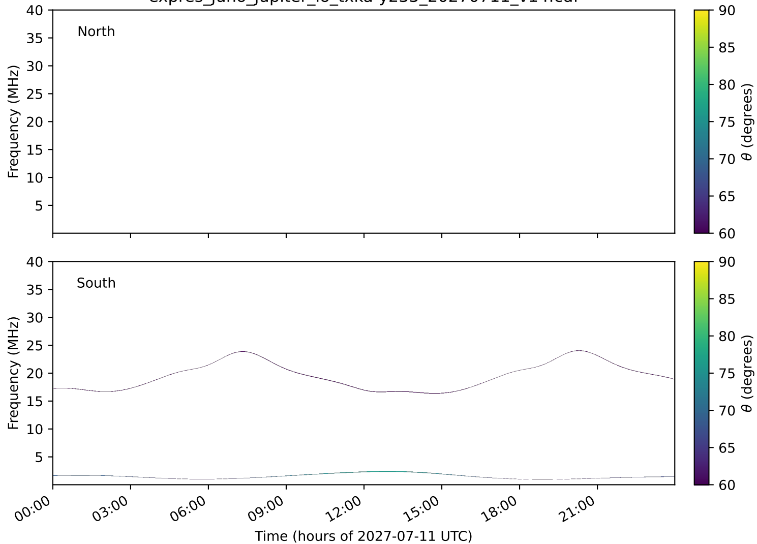
expres_juno_jupiter_io_txka-y235_20270711_v14.cdf
